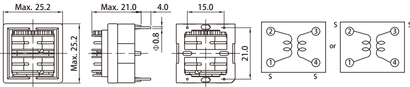
DIMENSIONS (mm)
