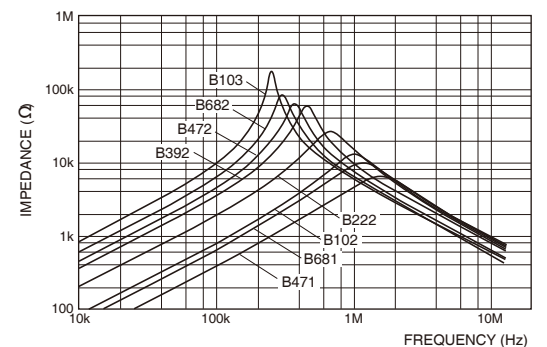
Impedance Characteristics
