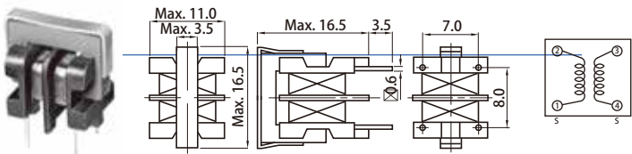
DIMENSIONS (mm)
