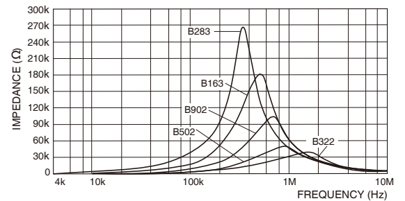
Impedance Characteristics
