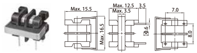
DIMENSIONS (mm)
